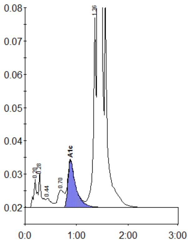
Peak table - ID: 10491233
